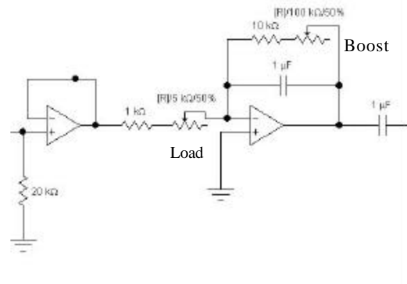
Fig. 4 - Boost Stage
