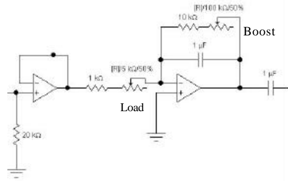
Fig. 4 - Boost Stage
